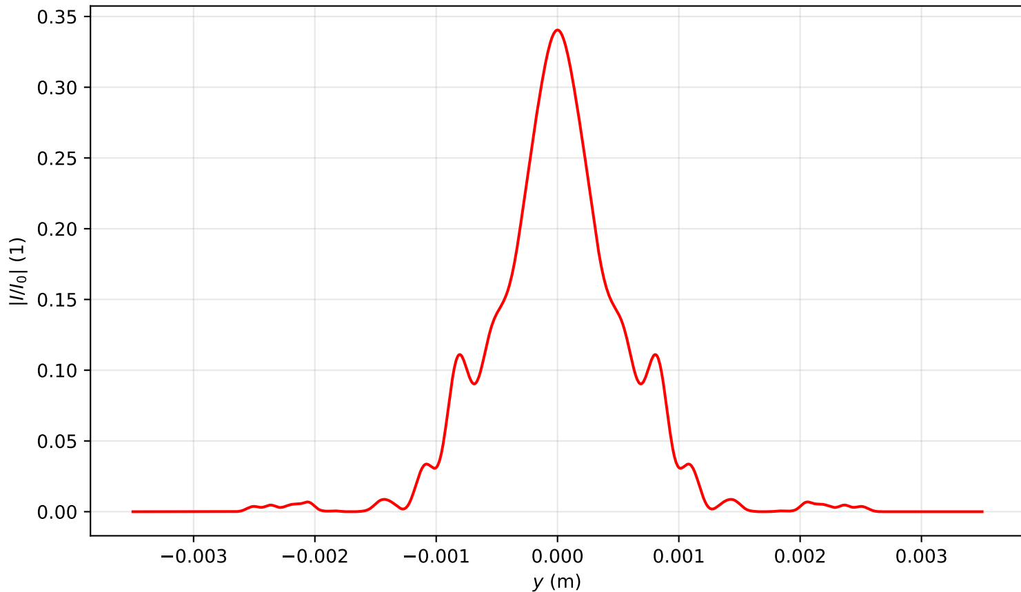
Intensity profile I(x=0, y, z=1.672)/I_0 , P_{in}=7.0P_{cr} , artificial time
